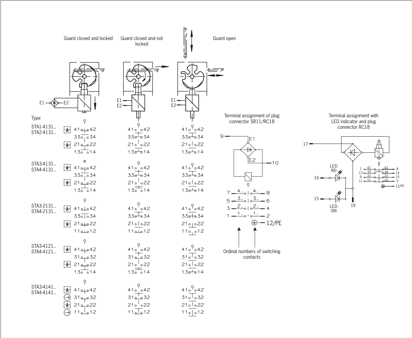
Fig. 3: Switching elements and switching functions
